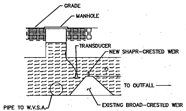
FLOODED CHAMBER
