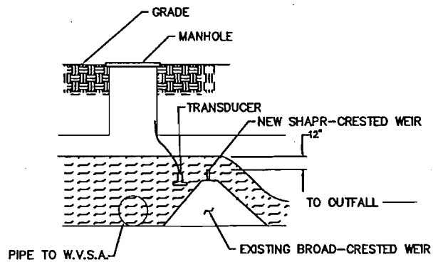
OVER FLOW BROAD-CRESTED WEIR WITH PLATE
