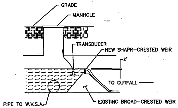
OVER FLOW SHARP-CRESTED WEIR
