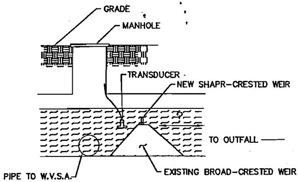
SUBMERGED WEIR
